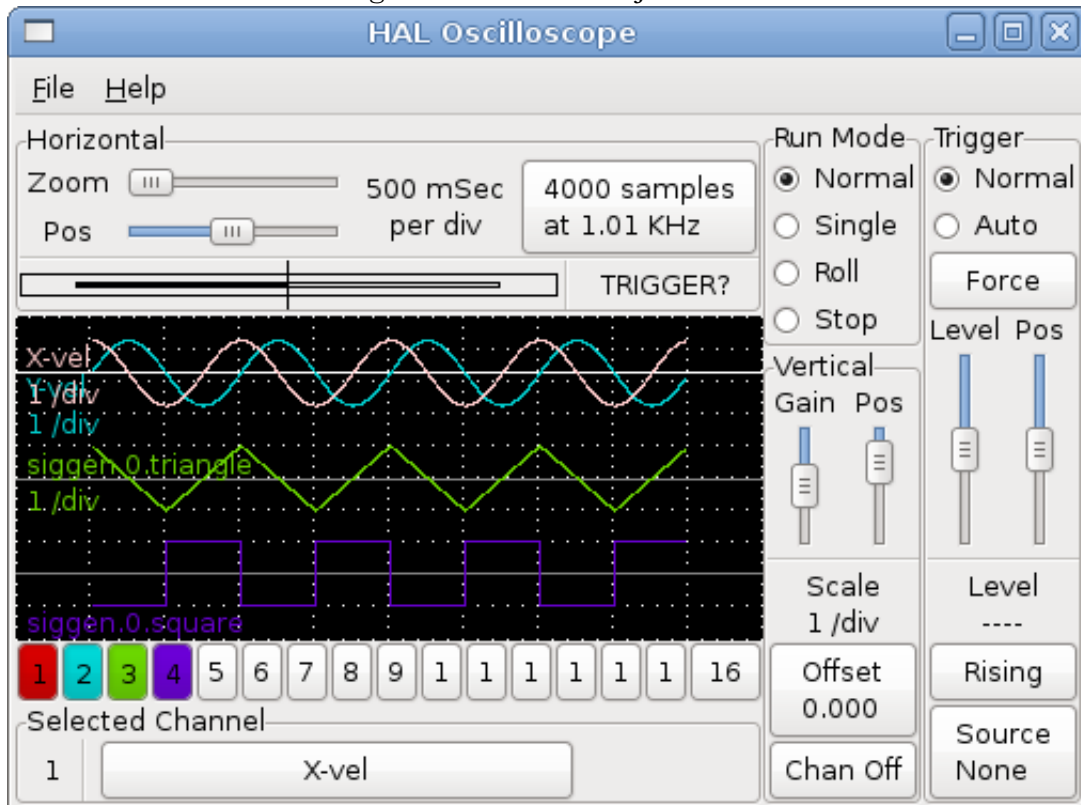
Figure 2.9: Vertical Adjustment
